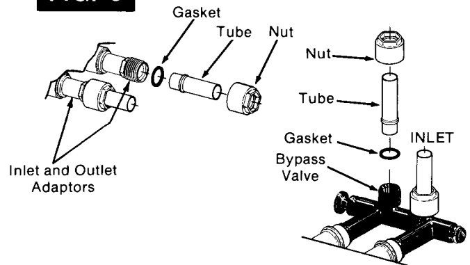
FIG. 8 INLET-OUTLET FITTINGS
