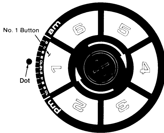
FIG. 18 TIME DIAL
