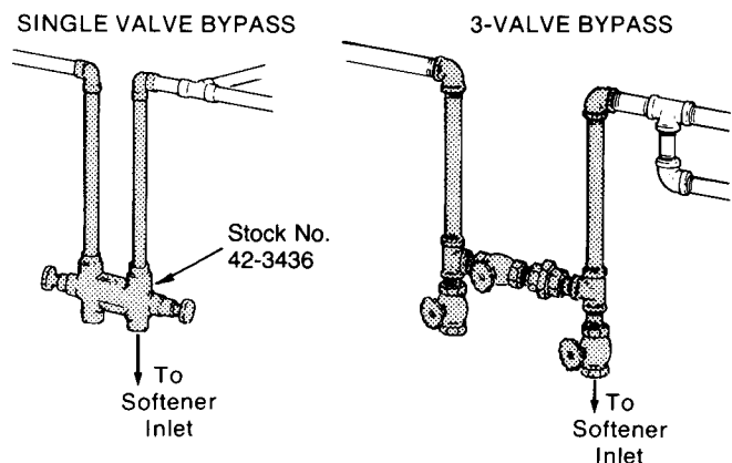
FIG. 7 BYPASS VALVES
