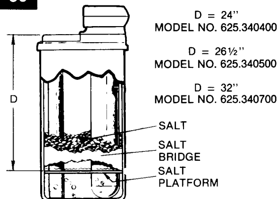
FIG. 30 A SALT BRIDGE
