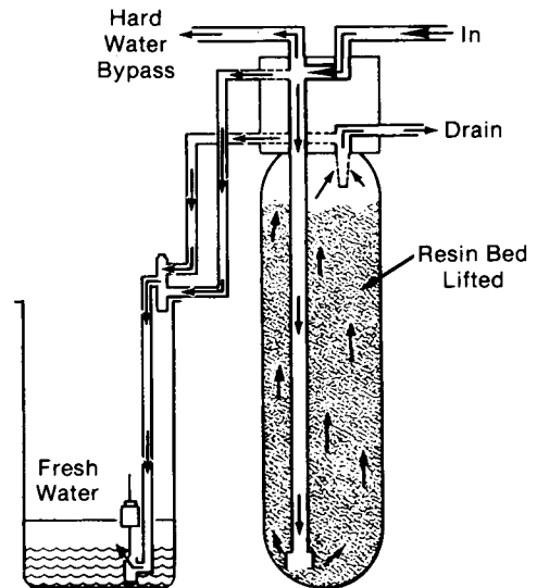
FIG. 21 WATER FLOW THROUGH THE SOFTENER IN BACKWASH
