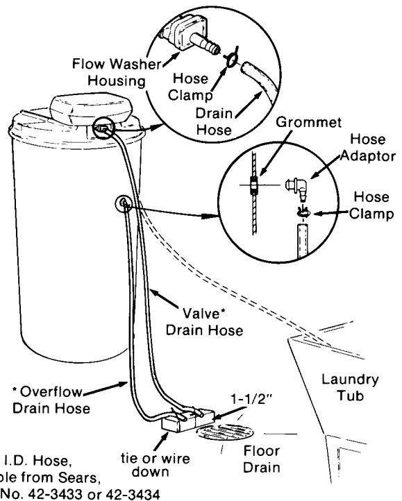
FIG. 10 SUMP — STANDPIPE DRAINS
